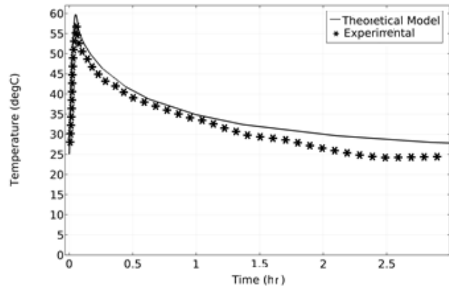
Fig 6 Variation of discharge temperature with time ( Q = 23 \text{ m}^3/\text{hr} )
