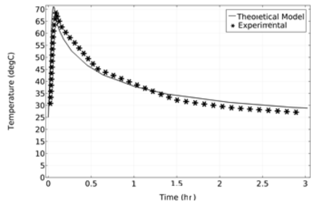
Fig 4 Variation of discharge temperature with time ( Q = 17 \text{ m}^3/\text{hr} )
