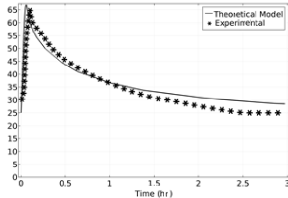
Fig 5 Variation of discharge temperature with time ( Q = 19 \text{ m}^3/\text{hr} )
